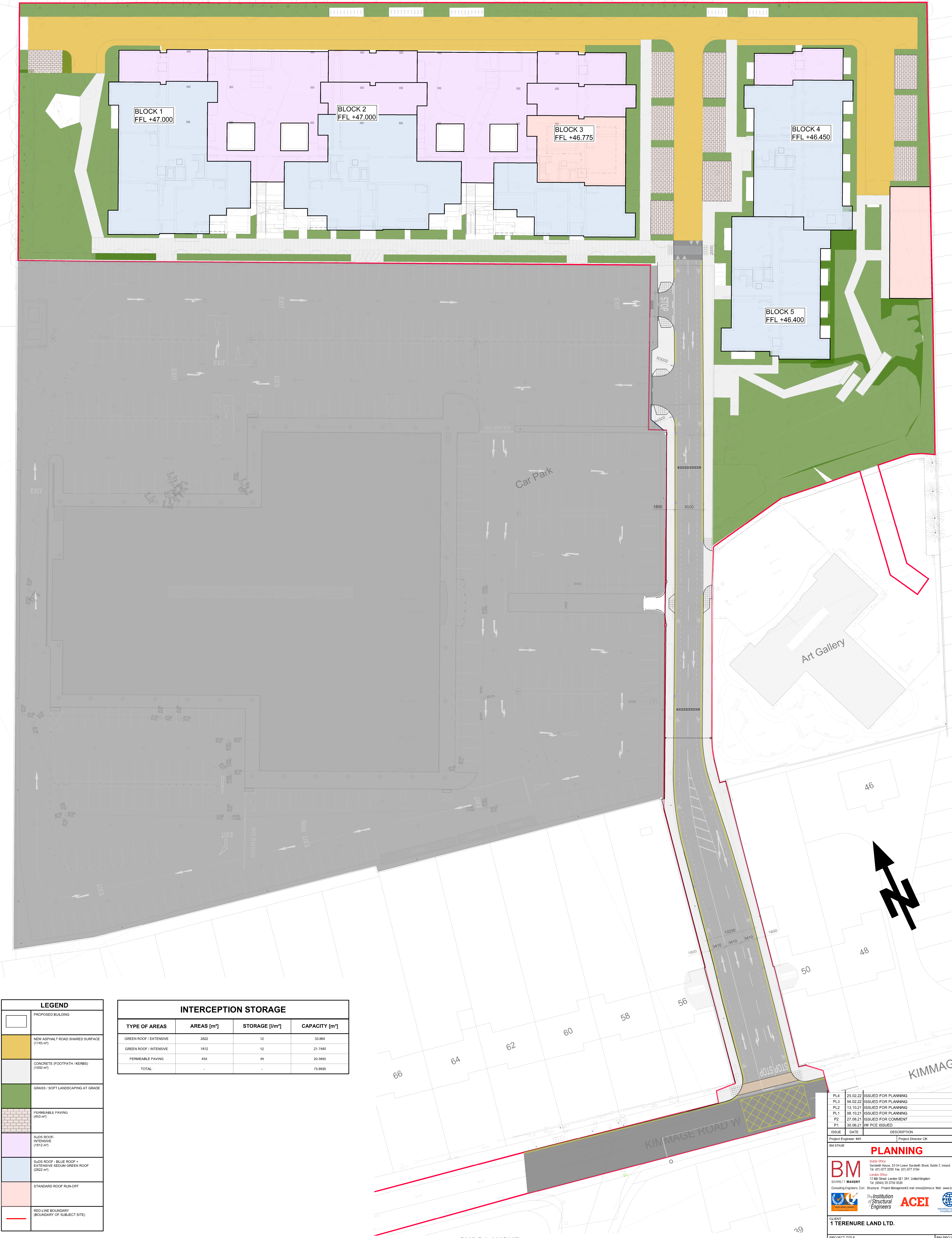
SUDS LAYOUT SCALE @ A0: 1:250 SCALE @ A2: 1:500
