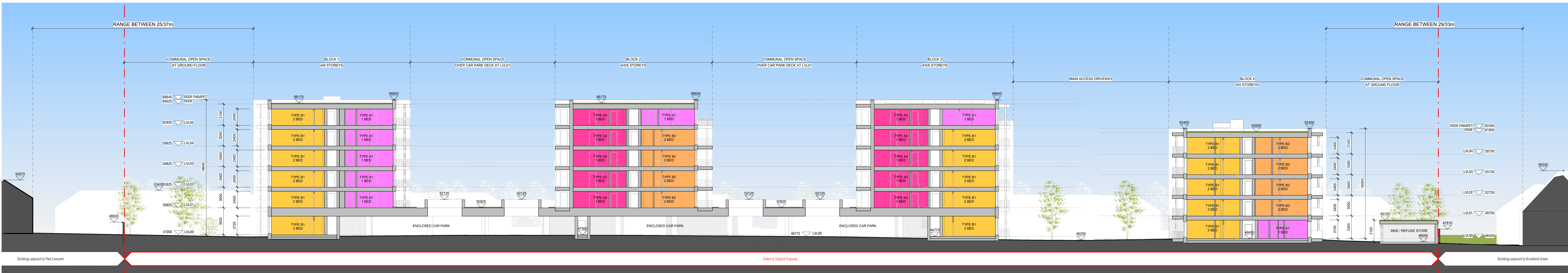
C Site Sections - Section C-C 1:200
