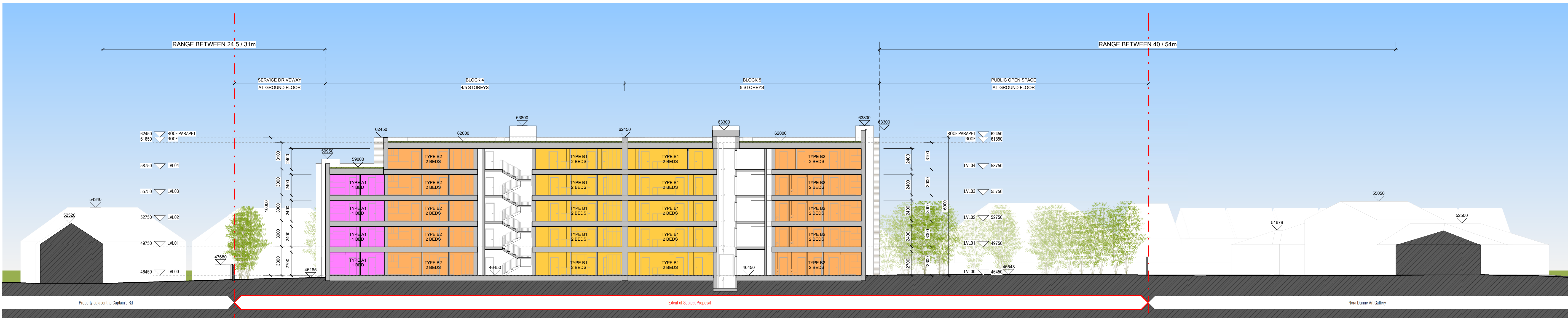
B Site Sections - Section B-B 1:200
